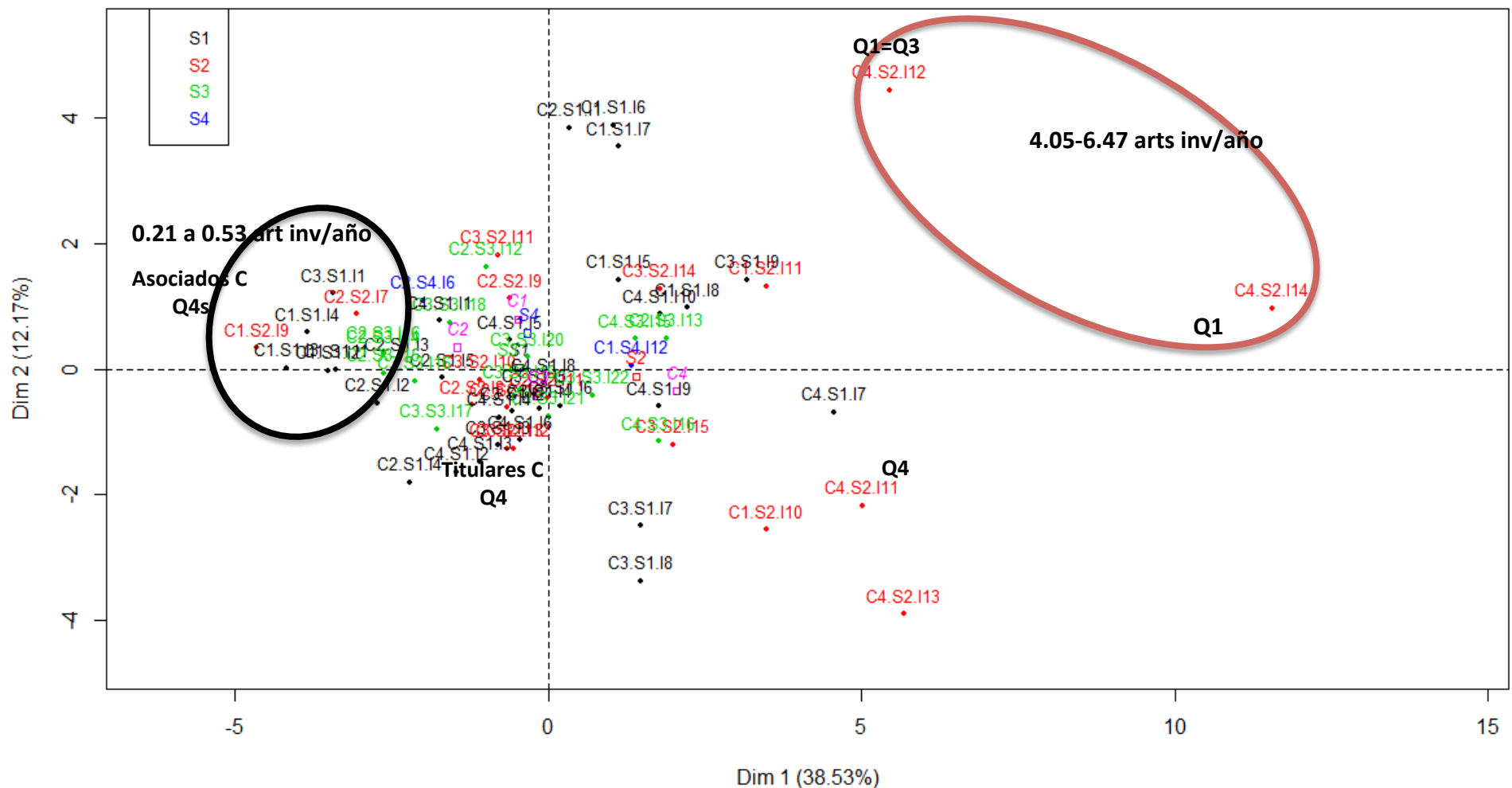
Individuals factor map (PCA)
